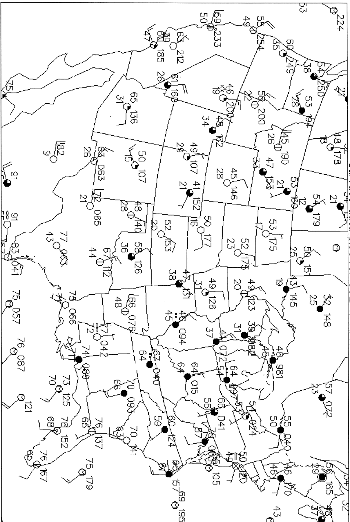
Surface data plot for 00Z 17 APR 98
